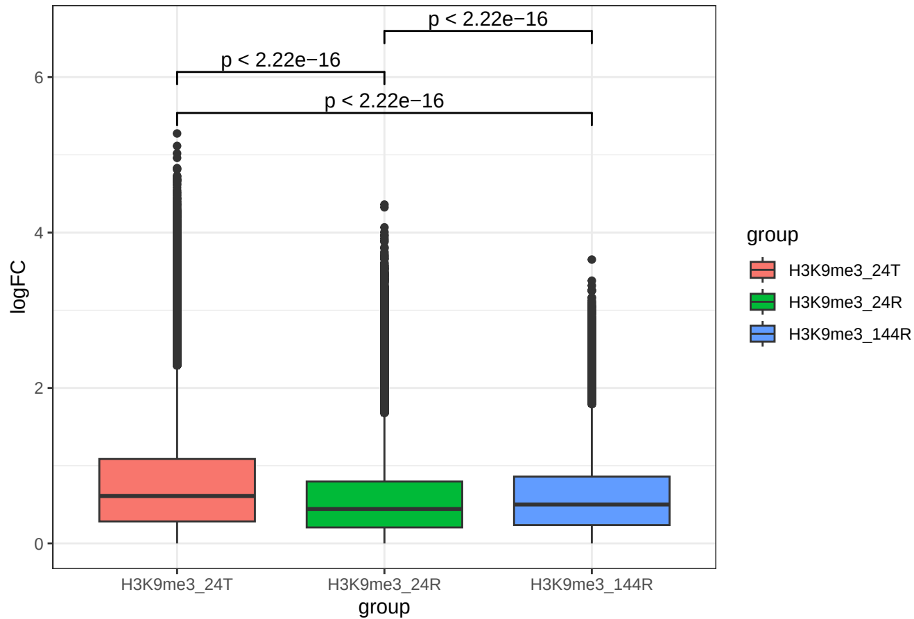
Absolute LFC across time for H3K9me3
